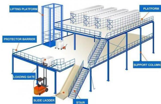
STAIRS AND HYDRAULIC LIFTING PLATFORMS The lifting platform is used to transport goods up and down between floors, with a large practical carrying capacity, smooth lifting and lowering, reducing manual handling, and slides can be configured according to needs.
